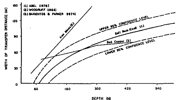
Figure 6: Transfer Distance vs. Depth.
