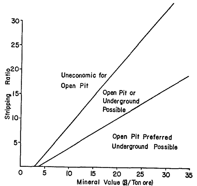
Figure 2: Stripping Ratio vs. Mineral Value.
