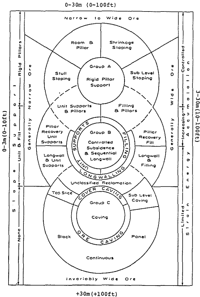
Figure 1: A Method Selection Scheme (after Morrison, 1976).
