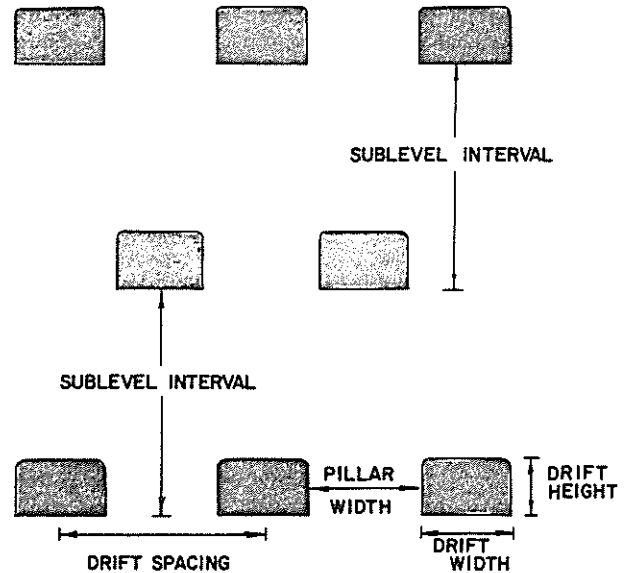
Figure 10: Sublevel Caving Geometry.
